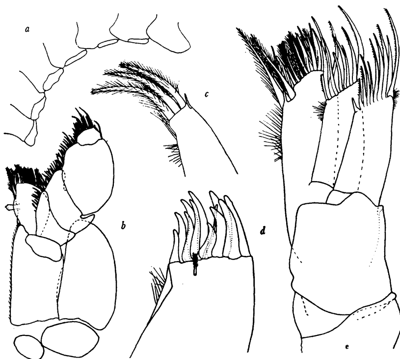
Fig. 2.— Pentidotea montereyensis , new species, a, right lateral side of thorax showing epimera. b, left maxilliped. c, left first maxilla, inner lobe. d, left first maxilla, outer lobe. e, left second maxilla.
