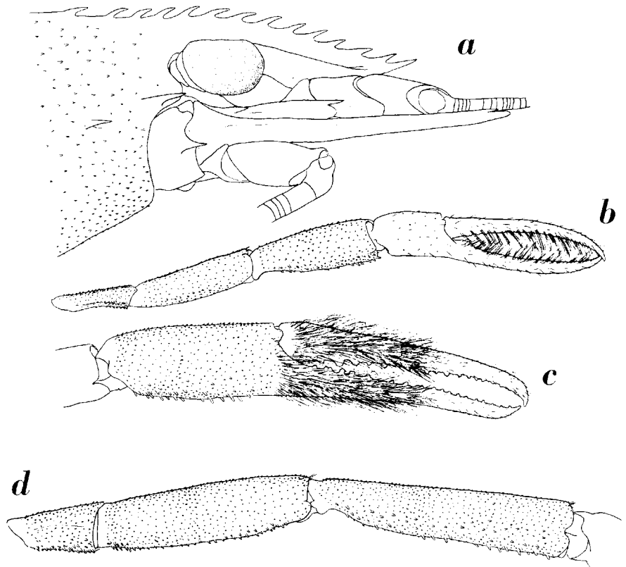
Fig. 5. Macrobrachium lorentzi (J. Roux, 1921), male from Ningerum, Papua New Guinea. a, anterior part of body in lateral view; b, smaller second leg; c, chela of larger second leg; d, ischium, merus and carpus of larger second leg. a, \times 6 ; b-d, \times 3 .
