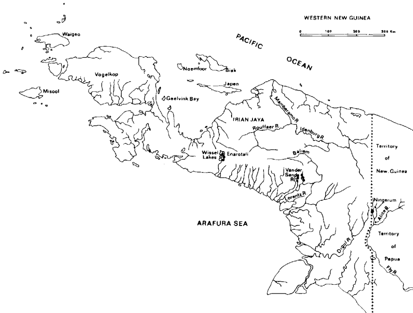
Fig. 6. Western New Guinea, showing the localities of Macrobrachium natulorum new species and M. lorentzi (J. Roux).
