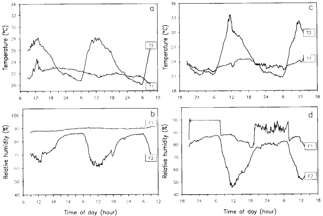
Fig. 4. Variation in temperature and relative humidity in the crevice system and at the forest floor measured in Discovery Bay near the coast (a, b) and at Windsor in central Jamaica (c, d). Temperature (T1) and relative humidity (F1) = measurement from crevice system; T2 and F2 = measurement from forest floor.
