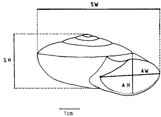
Fig. 2. Shell of Pleurodonte lucerna ; position of standard measurements. SW = shell width; SH = shell height; AW = aperture width; AH = aperture height.
