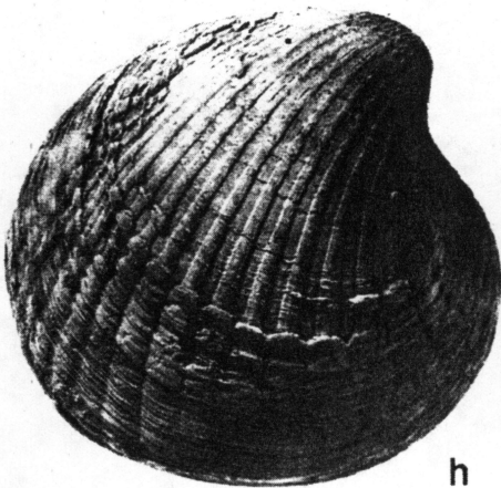
Figure 2. Representative macrofossils from the marine "Stewart bed" of the Llajas formation, north side of Simi Valley. All specimens are the same ones used in Squires (1984); a) typical exposure of the "Stewart bed"; b) solitary coral, Trochocyathus striatus , height 36 mm; c) scaphopod, Dentalium stentor , height 76 mm; d) snail, Turritella andersoni lawsoni , height 38 mm; e) snail, Eocernina hannibali , height 47 mm; f) snail, Cymatium (Septa) janetae , height 43 mm; g) snail, Ficopsis remondii crescentensis , height 43 mm; h) clam, Venericardia (Pacifcor) hornii calafia , height 110 mm; i) clam, " Crassatella " ucasana , height 58 mm; j) nautiloid, Aturia myrlae , height 26 mm; k) shark tooth, Odontaspis sp., height 32 mm.
