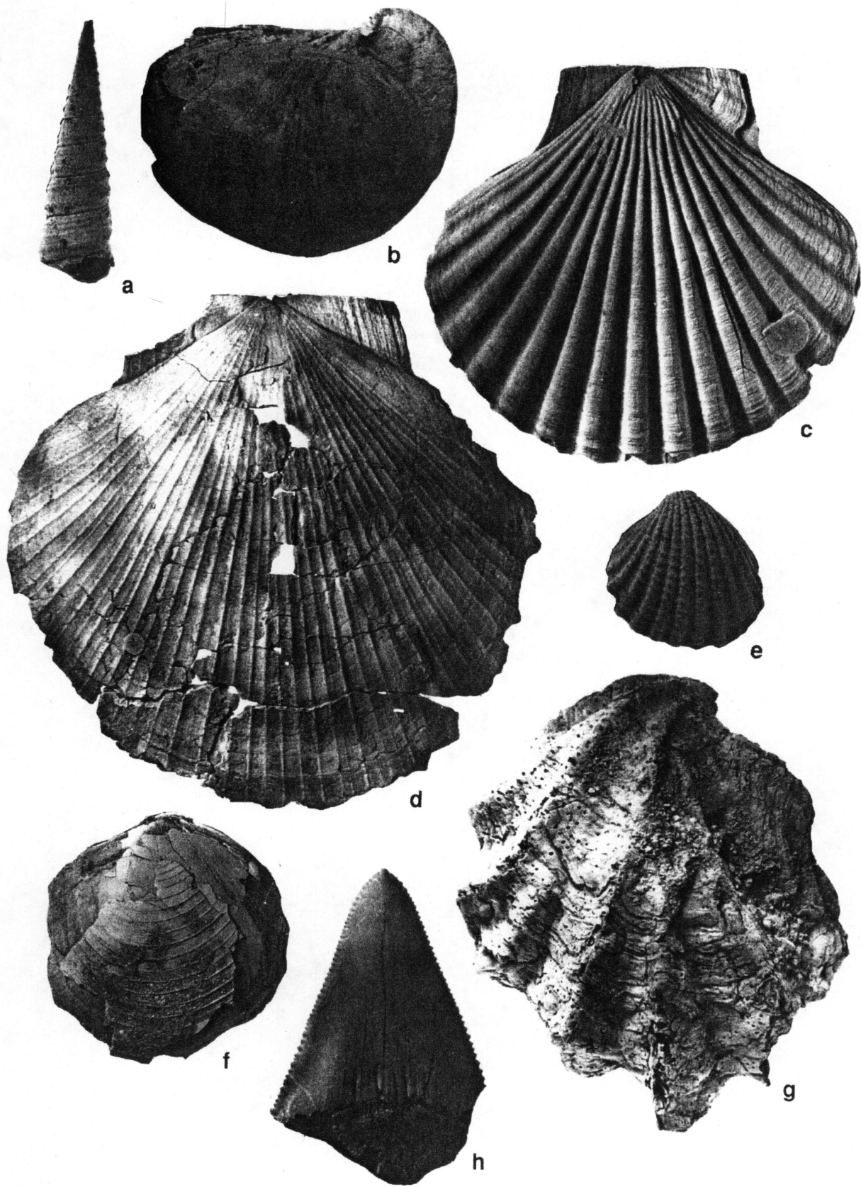
Figure 6. Representative macrofossil from the marine part of the Saugus Formation, north side of Simi Valley. All specimens are the ones used in Squires and White 1983 in Squires and Filewicz 1983; a) snail Turritella cooperi , height 33 mm; b) snail Crepidula princeps , width 90 mm; c) clam Pecten (Pecten) bellus , height 55 mm; d) Patinopecten healeyi , height 156 mm; e) clam Cyclocardia occidentalis , height 18 mm; f) clam Lucina (Lucinoma) annulata , height 52 mm; g) clam Dendostrea vespertina , height 86 mm; h) great-white shark tooth Carcharodon sp., height 60 mm.
