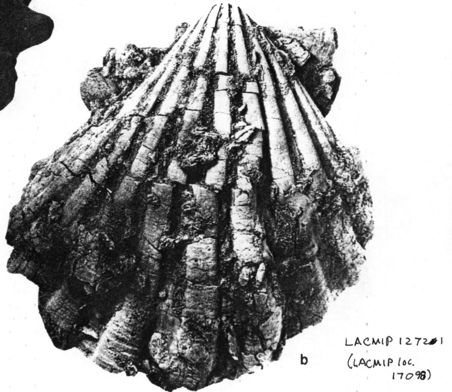
Figure 4. Two representative macrofossils from the Vaqueros Formation, Big Mountain Oil Field area, north side of Simi Valley. Both specimens photographed by R. L. Squires; a) snail Rapana vaquerosensis imperialis , height 100 mm; b) clam Macrochlamis magnolia , height 130 mm.
