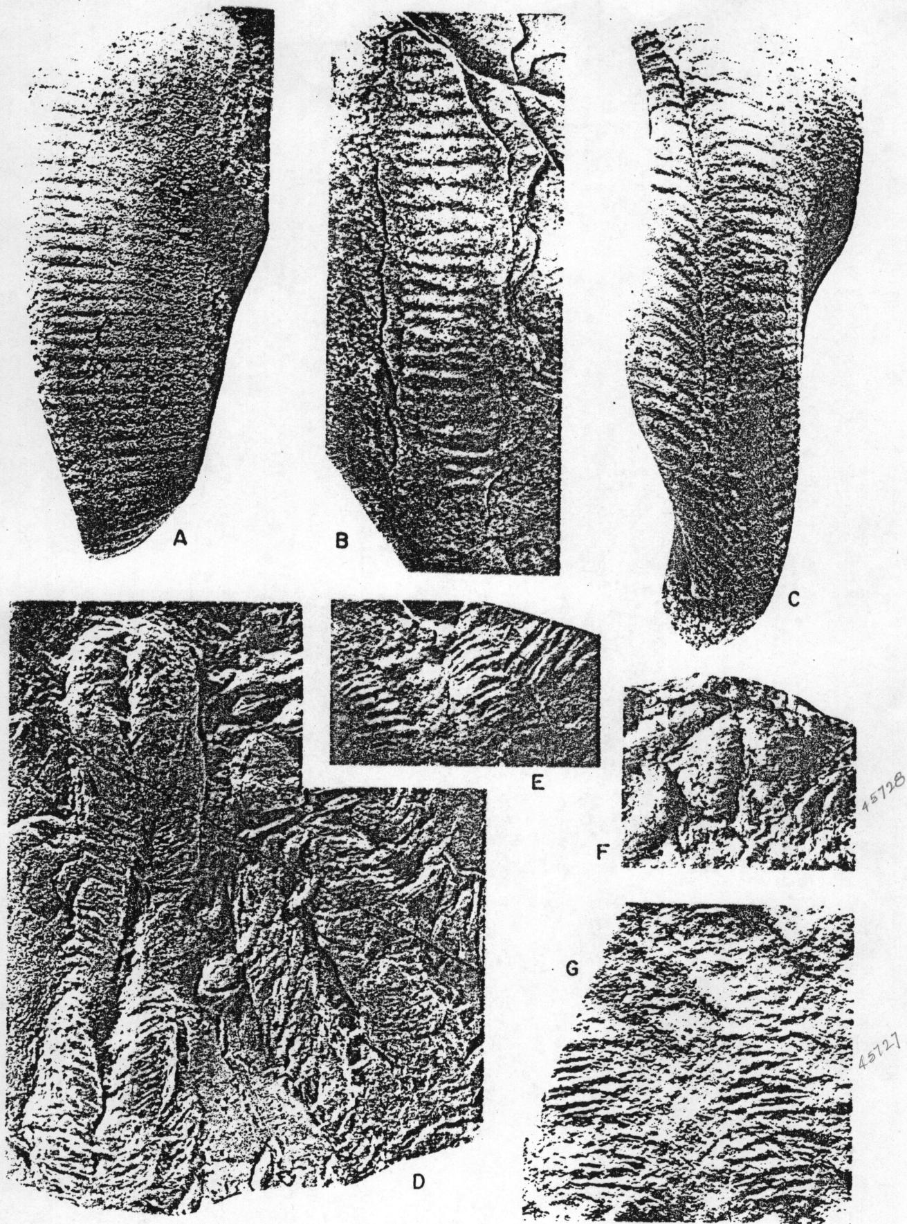
PLATE 1. -- A, C - Pteridinium simplex Gürich, Kuibis quartzite, base of Nama System, South West Africa. B - cf. Pteridinium , Middle mem., Deep Spring Fm., loc. 7, Fig. 2B. D - Rusophycus-Cruziana , Middle Cambrian Tapeats Ss., Grand Canyon. E, G - Cruziana , Upper mem., Deep Spring Fm., loc. 1, Fig. 2A. F - Rusophycus , same loc. as E, G. Plate from Cloud and Nelson (1966). Figures approximately natural size.
