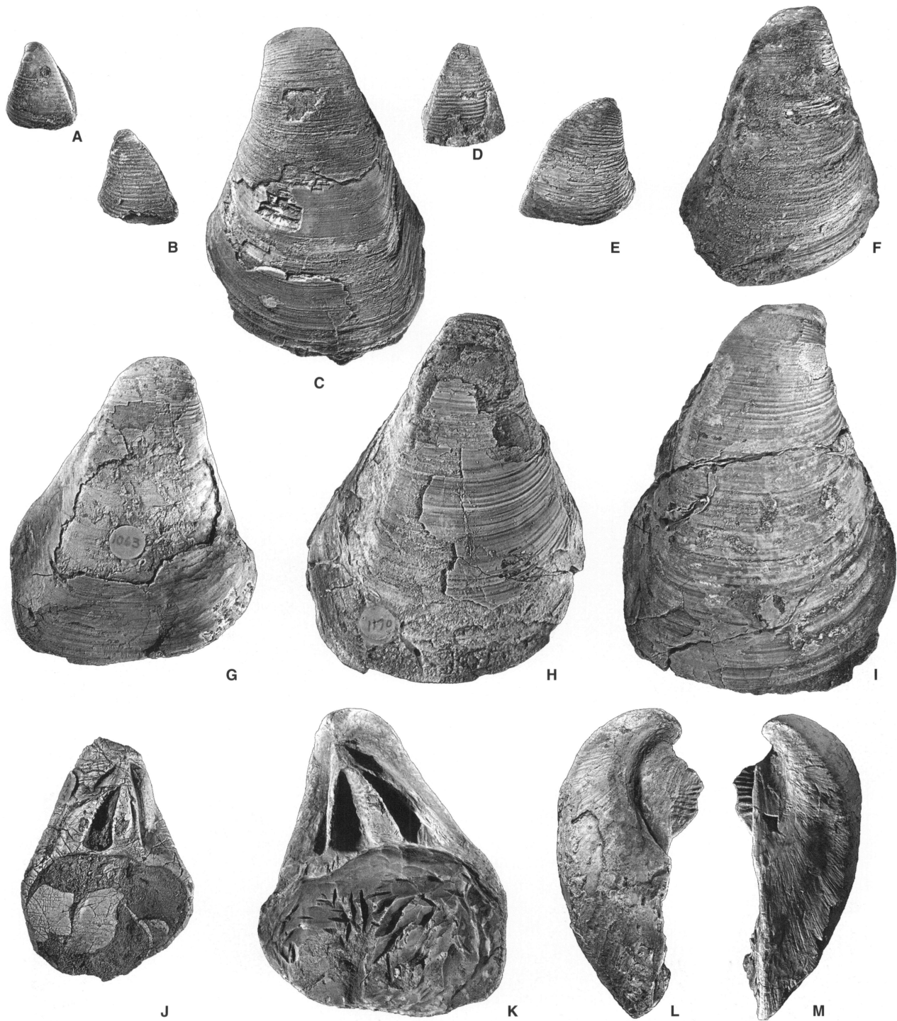
TEXT-FIG. 8. Figs 1–20. Opis (Hesperopis) anae sp. nov. All \times 1 . Specimens coated with ammonium chloride. A, paratype, LACMIP 13525, LACMIP loc. 10718, left valve. B, paratype, LACMIP 13526, LACMIP loc. 10724, left valve. C, paratype, LACMIP 13527, LACMIP loc. 22329, left valve. D, paratype, LACMIP 13528, LACMIP loc. 10724, right valve. E, paratype, LACMIP 13529, LACMIP loc. 10724, right valve. F, paratype, LACMIP 13530, LACMIP loc. 8173, right valve. G, K–M, holotype, LACMIP 13531, LACMIP loc. 10718, right valve. G, exterior. K, interior. L, lunule view. M, escutcheon/corcelet view. H, paratype, LACMIP 9917, LACMIP loc. 10084, right valve. I, paratype, LACMIP 13532, LACMIP loc. 22329, right valve. J, paratype, LACMIP 13533, LACMIP loc. 22329, left-valve interior.
