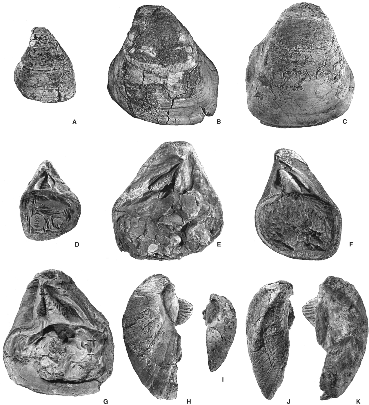
TEXT-FIG. 6. Opis ( Hesperopis ) holzana sp. nov. All specimens, unless otherwise noted, from LACMIP loc. 24190. All \times 1 . Specimens coated with ammonium chloride. A, D, I, paratype, LACMIP 13522, left valve. A, exterior. D, interior. I, lunule view. B, E, J, paratype, LACMIP 13523, left valve. B, exterior. E, interior. J, escutcheon/corcelet view. C, G-H, K, holotype, LACMIP 13524, right valve. C, exterior. G, interior. H, lunule view. K, escutcheon/corcelet view. F, paratype, RBCM.EH2008.016.0001, right-valve interior, CGS loc. 103851.
