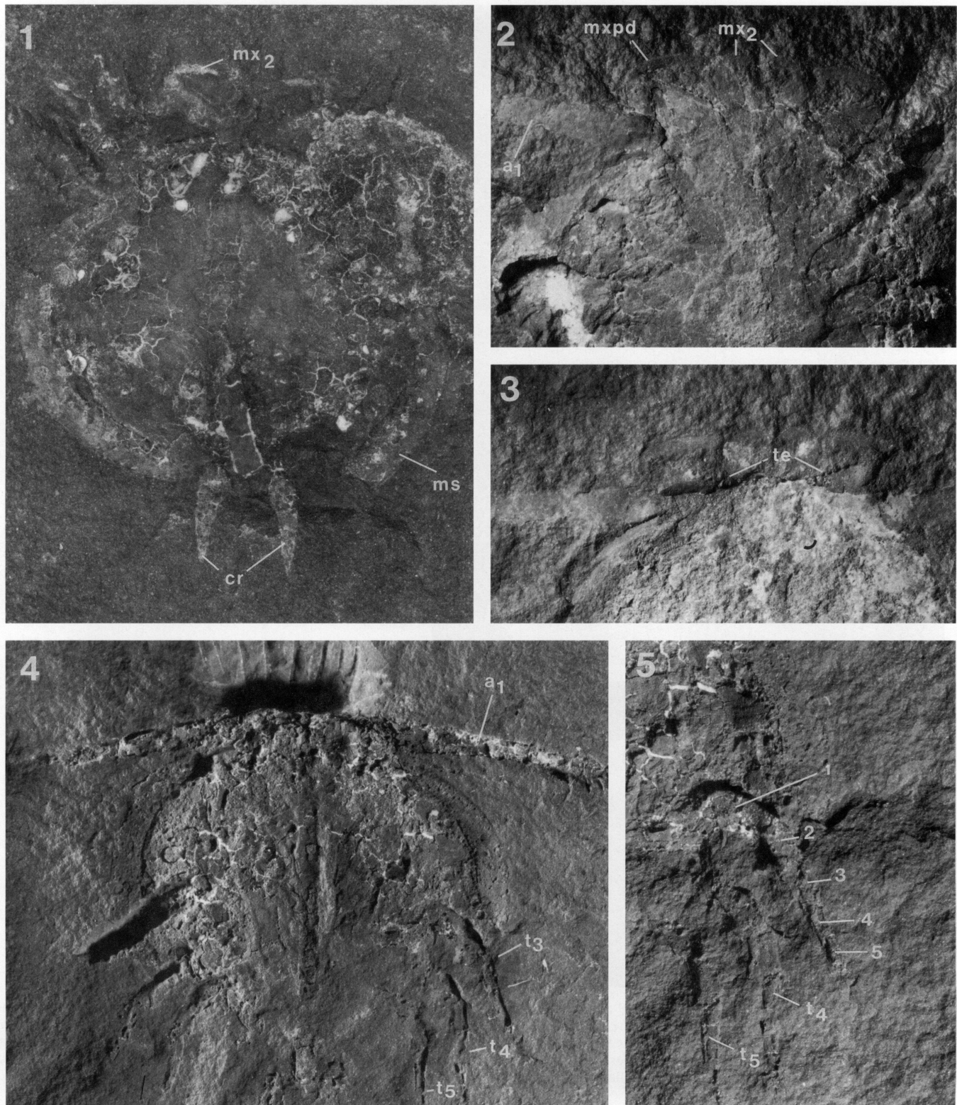
FIGURE 5— Cyclus americanus Packard. 1, PE 22421 with maxillary geniculum extended to display scimitar-like terminal segment, blade-like penultimate segment, and caudal rami, \times 5 . 2, 3, PE 34954 (part and counterpart) \times 4.8 , 2, Medial-most maxillary genicula and maxillipede distal segment. 3, Clear view of teeth on penultimate blade of maxillipedal genicula. 4, 5, PE 34759, 4, Showing general body form and placement of thoracic legs, \times 4.3 . 5, Close-up revealing leg segments distal to knee, \times 7.8 . a1 = antennule, cr = caudal rami, ms = marginal shelf of carapace, mx2 = maxillae, te = teeth, t "n" = thoracopods, 1–5 segments on third thoracopod.
