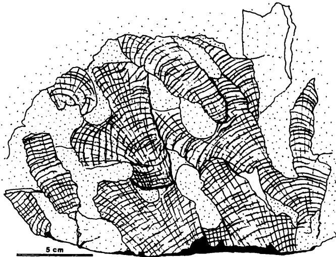
FIGURE 3—Line drawing of the flattened holotype of Farrea rugosa new species, LACMIP 12244, shows patterns and distributions of bifurcations and branches of the structure, as well as some of the wrinkles. Preserved edges of individual branches and bifurcations that appear to be part of a single larger branch are shown in somewhat heavier lines. Matrix between branches is lightly stippled. Bar scale at the base shows dimensions of the exposed sponge.
