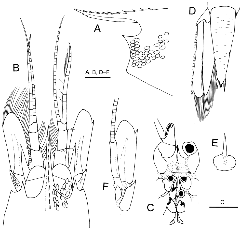
Fig. 2. Bresilia ruficulus sp. nov., holotype, ovigerous female (cl 2.1 mm), CBM-ZC 10063. A, rostrum and anterior part of carapace, lateral view; B, rostrum, anterior part of carapace and cephalic appendages, dorsal view (tegumental scales are partially illustrated); C, fifth to eighth thoracic sternites, ventral view (appendages were removed); D, telson and left uropod, dorsal view; E, epistome, ventral view; F, left antenna, ventral view. Scale bars: 0.5 mm.
