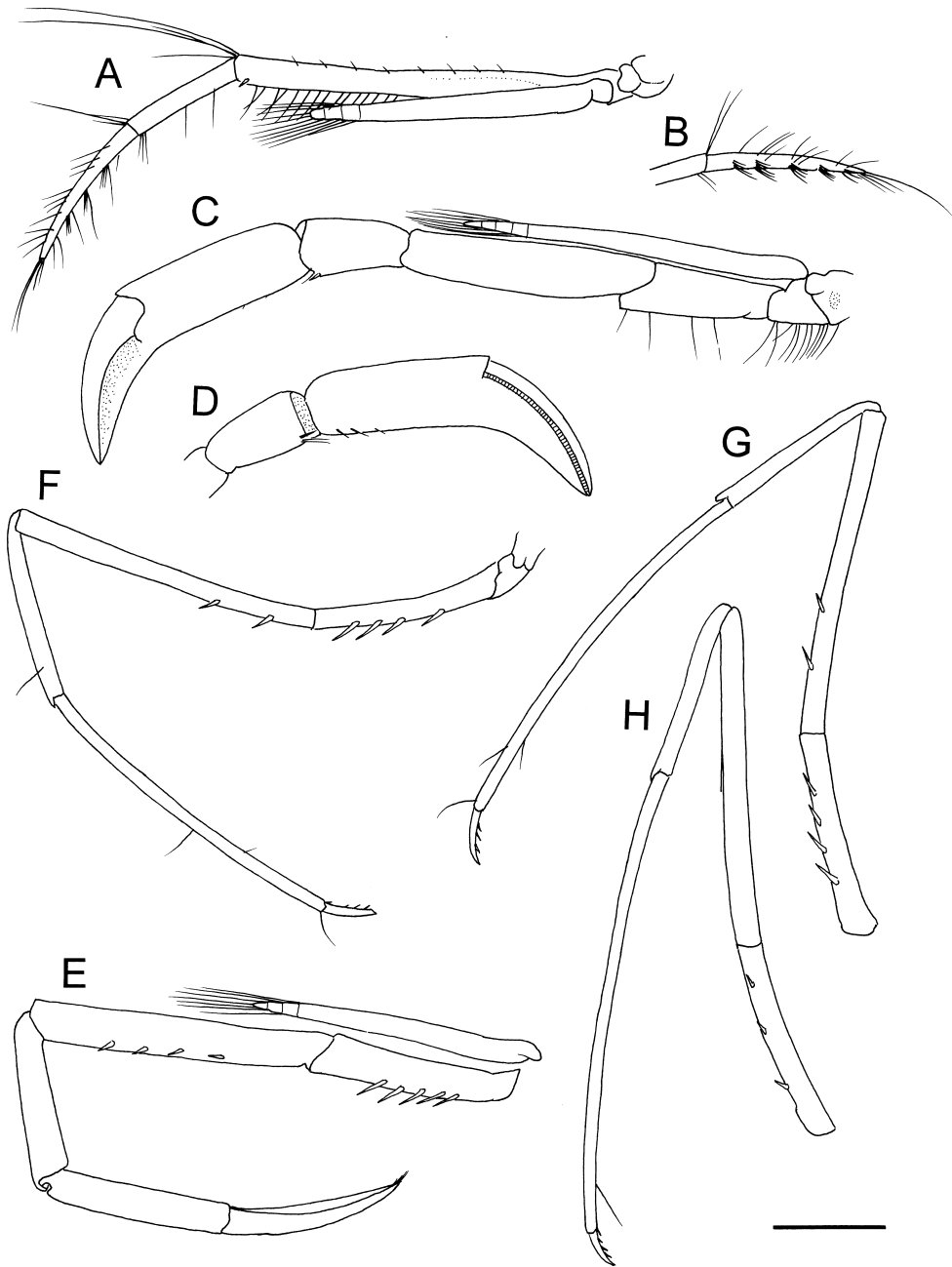
Fig. 4. Bresilia rufioculus sp. nov., holotype, ovigerous female (cl 2.1 mm), CBM-ZC 10063, left thoracic appendages. A, third maxilliped, lateral view; B, same, ultimate segment, mesial view; C, first pereopod, lateral view; D, same, chela and carpus, mesial view; E, second pereopod, lateral view; F, third pereopod, lateral view (tip of dactylus is broken off); G, fourth pereopod, lateral view; H, fifth pereopod, lateral view. Scale bar: 0.5 mm.
