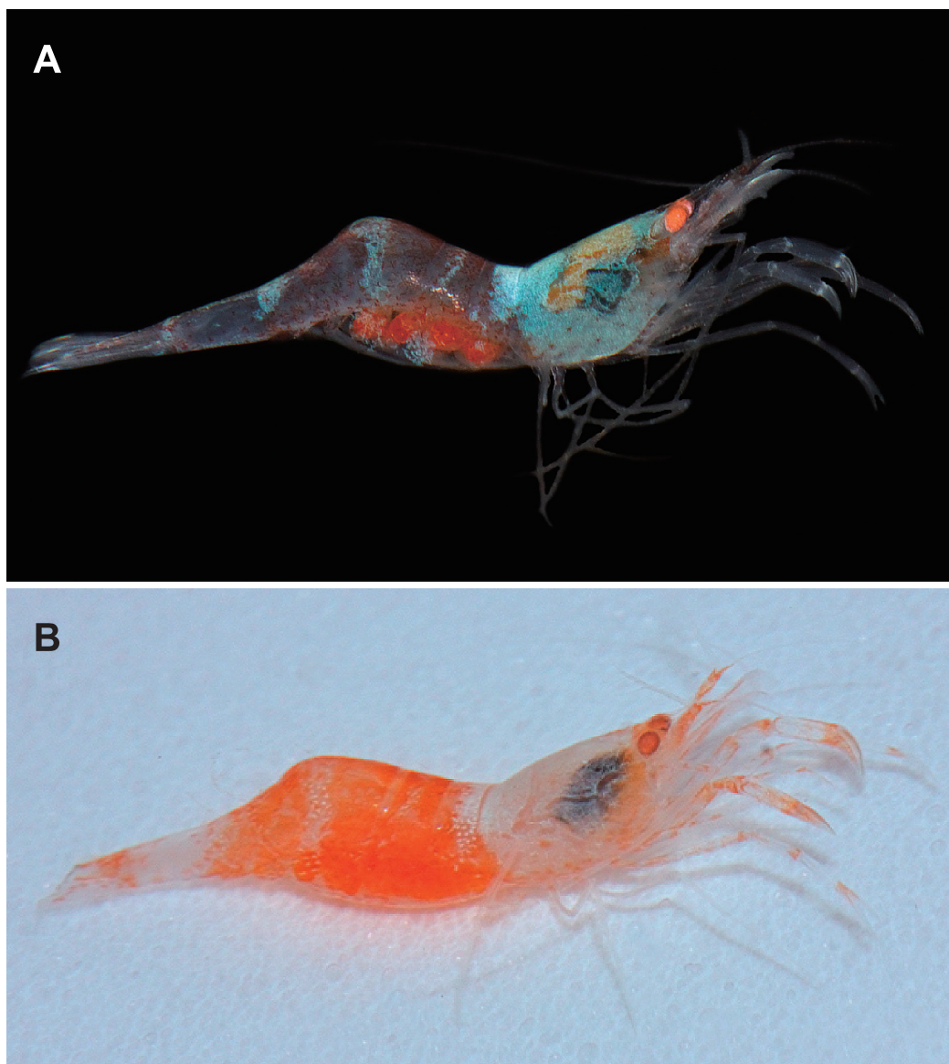
Fig. 6. Bresilia rufulioculus sp. nov., photographs showing color in life. A, holotype, ovigerous female (cl 2.1 mm), CBM-ZC 10063; B, paratype, ovigerous female (cl 2.3 mm), NSMT-Cr 21341.
