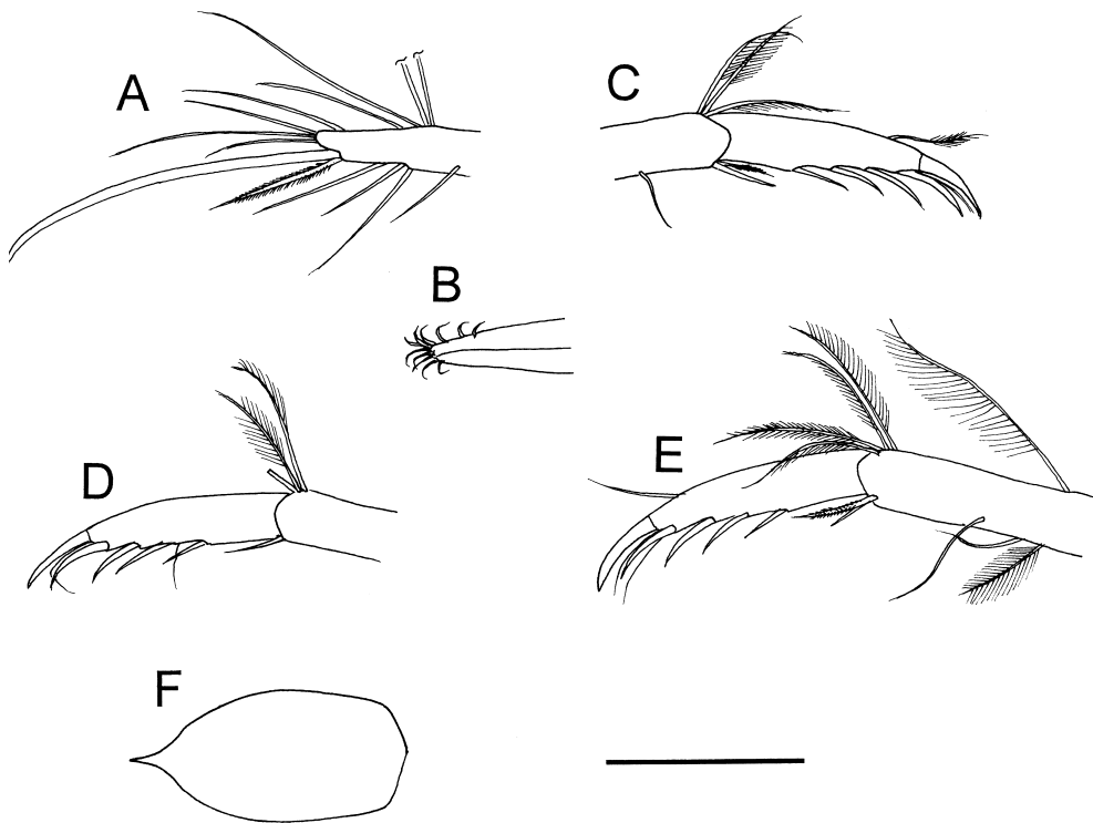
Fig. 5. Bresilia rufiocus sp. nov., holotype, ovigerous female (cl 2.1 mm), CBM-ZC 10063. A, detail of tip of ultimate segment of left third maxilliped, lateral view; B, detail of tip of fingers of left second pereopod; C, dactylus and distal part of propodus of right third pereopod, lateral view; D, dactylus and distal part of propodus of left fourth pereopod, lateral view; E, dactylus and distal part of propodus of left fifth pereopod, lateral view; F, tegumental scale removed from lateral face of carapace. Scale bar: 0.2 mm for A–E; 0.1 mm for F.
