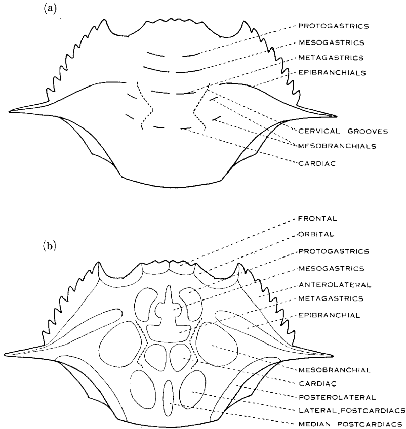
Fig. 1.—(a) Designation of ridges and depressions of carapace in species of Portunus without elevated areas (depressions dotted).
