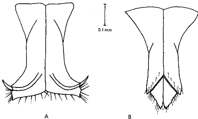
Fig. 2. Adult male operculum of (A) Jaera albifrons ischioisetosa (body length 1.5 mm) and (B) J. nordmanni nordica (body length 2.8 mm).
