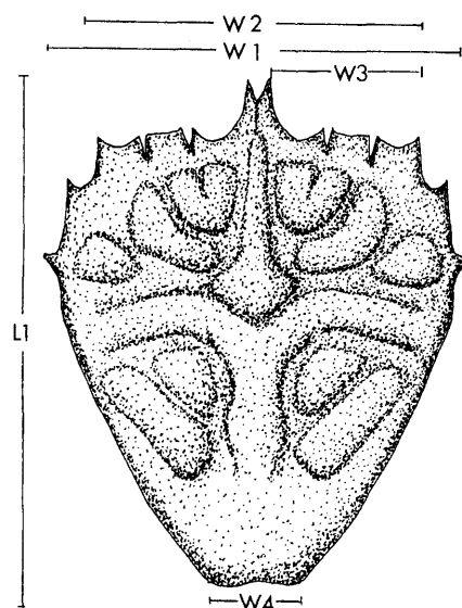
Fig. 16. Line drawing of Eucorystes platys sp. nov., showing the position and orientation of measurements taken.
