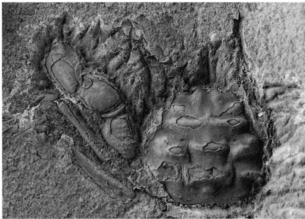
Fig. 19. Archaeopus vancouverensis (Woodward, 1896), dorsal carapace, USNM 512169. Scale bar equal to 1 cm.
