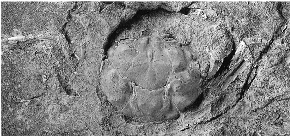
Fig. 17. Archaeopus lunicarina sp. nov. 1, dorsal carapace, holotype, UAM2574a. 2, chela, paratype, UAM2576. 3, dorsal carapace, rounded morphology, paratype, UAM2581. Scale bar equal to 1 cm.
