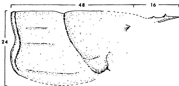
Fig. 8. Line drawing of Nephropidae, genus indeterminate, USNM 512161, showing the position and values of measurements taken (mm).
