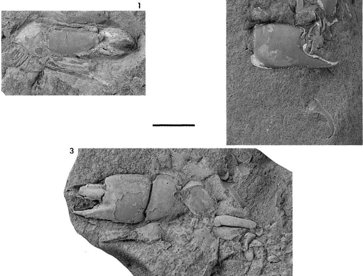
Fig 9. 1, Brecanclawu rathbunae gen. nov. and sp. nov., major and minor chelae, holotype, USNM 512170. 2, Callianassa s.l. sp., UAM 2686. 3, Callianopsis ? inornatus sp. nov., holotype, USNM 512168. Scale bar equal to 1 cm.
