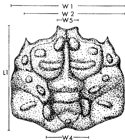
Fig. 18. Line drawing of Archaeopus lunicarina sp. nov., showing the position and orientation of measurements taken.
