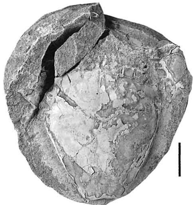
Fig. 15. Eucorystes platys sp. nov., dorsal carapace, holotype, USNM 512163. Scale bar equal to 1 cm.
